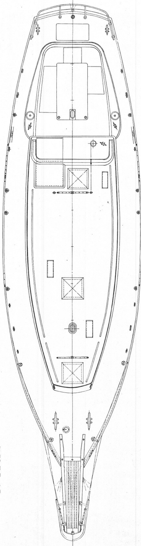
FUJI 45 MARK I DECK PLAN SCALE 1/8" = 1'-0"
